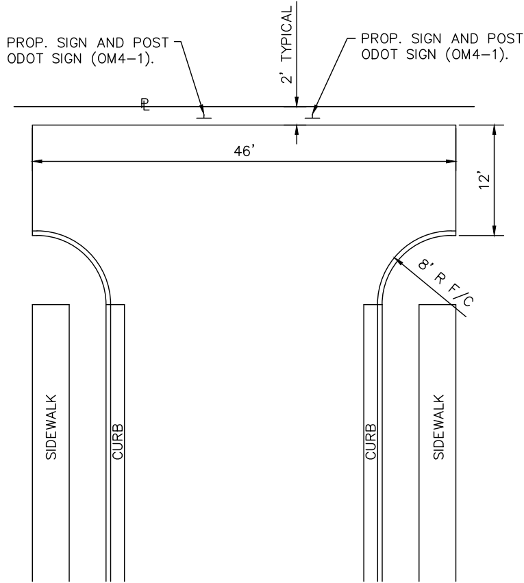
TEMPORARY HAMMER HEAD
