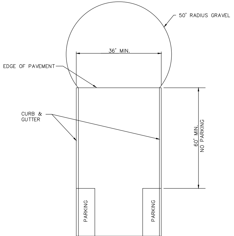
TEMPORARY DEAD-END STREETS
