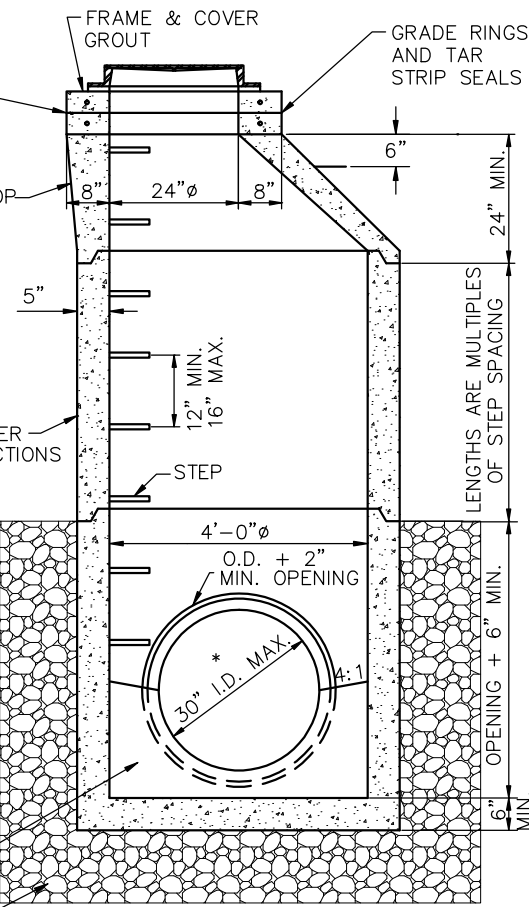
48" PRECAST BASE FOR 30" & SMALLER PIPE
