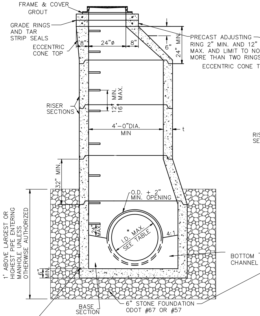
60" TO 96" PRECAST BASE SEE TABLE FOR MAXIMUM PIPE SIZES
