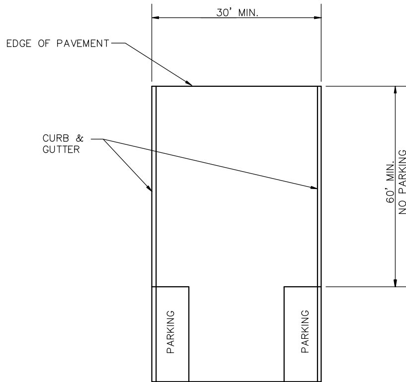
TEMPORARY DEAD-END STREETS
