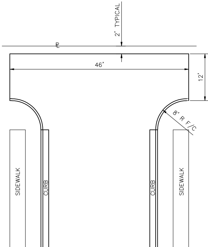
TEMPORARY HAMMER HEAD
